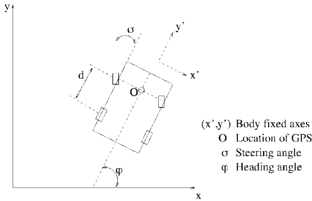
Figure 13. The “bicycle” model.
