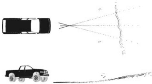
Figure 6. Ladders distinguish obstacles from the ground surface.
