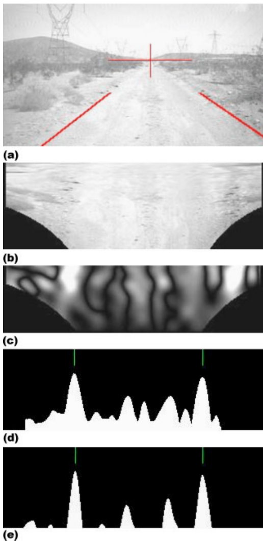
Figure 16. Projection-warp search: (a) Original image with the overlaid path boundary and focus of expansion results, (b) the warped image, (c) texture gradients magnitude, (d) projection: Vertical sum of gradients, and (e) projection profile followed by convolution with a box filter. The two lines on top of the histogram mark the path boundaries.
