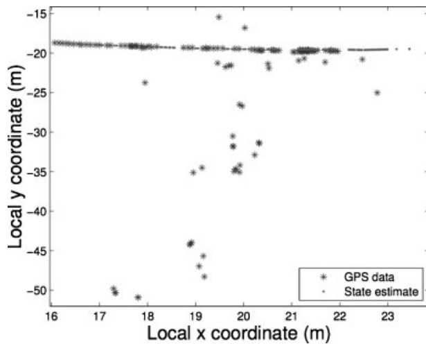
Figure 14. Performance of state estimator while going under a bridge.
