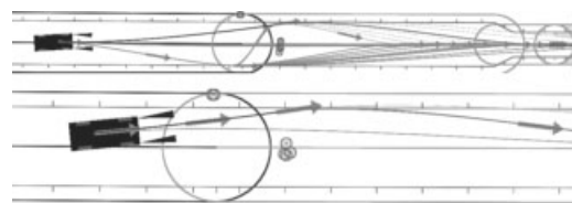
Figure 11. Visualization of Avoider graph as the vehicle navigates around a tank trap obstacle during the NQE.
