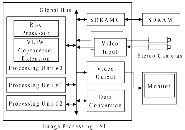
Figure 22. Block diagram of Visconti.
