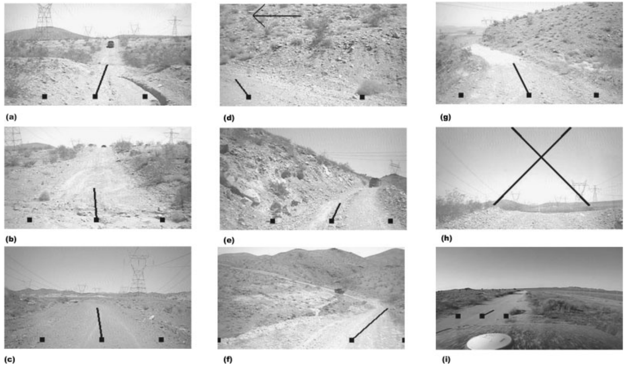
Figure 18. Sample images and system output from 6 h of driving in the Mojave desert. The path is marked by two left-right boundary points and a center point with heading orientation. The “X” mark in (h) coincides with zero confidence due to short range of visible path. In (i), the path is detected even though the vehicle is not centered on the path (a common situation in autonomous driving).
