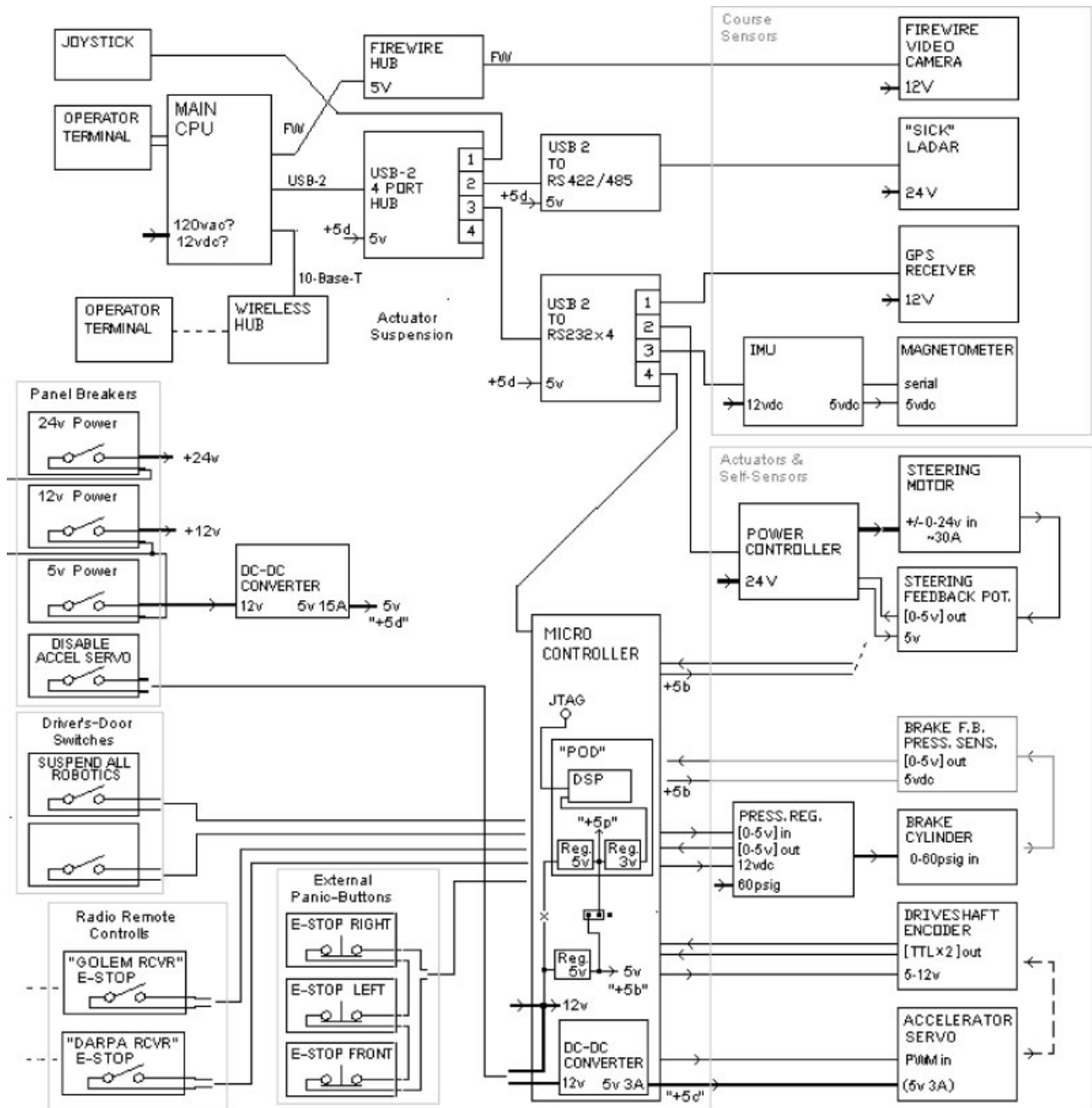
Figure 3. Block diagram of the Golem vehicle architecture.
