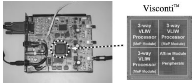
Figure 21. Prototype processing hardware.
