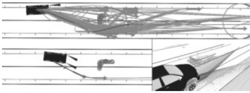
Figure 12. Visualization of Avoider graph as the vehicle navigates around a parked car obstacle during the NQE.
