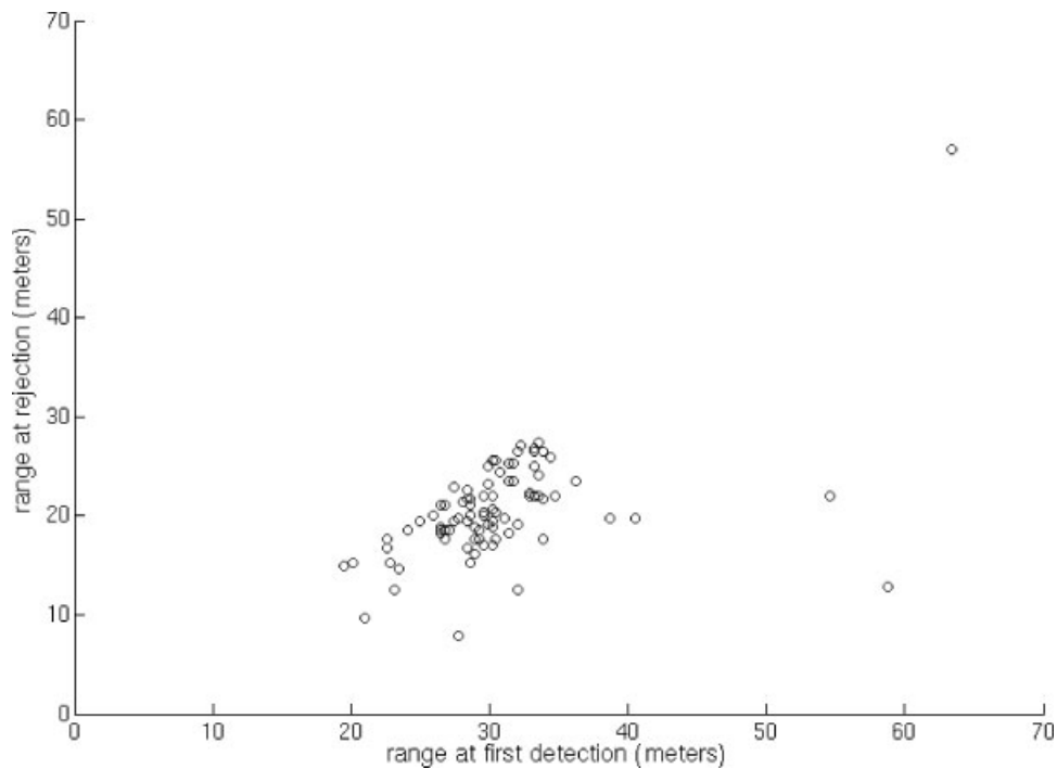
Figure 9. False positive events in which obstacles were “detected,” but subsequently rejected.
