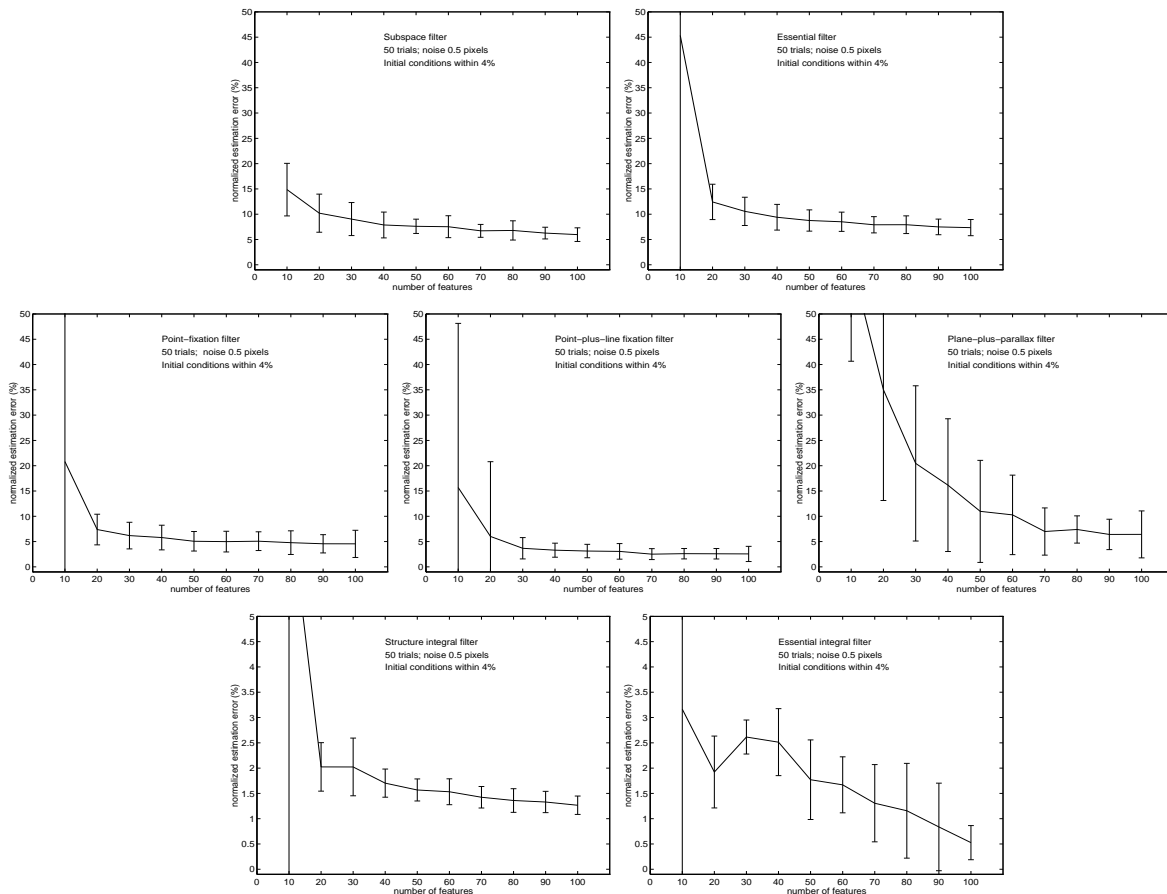
Figure 6: Dependence upon the number of features. The norm of the estimation error is plotted against the number of visible features, for a noise level of half a pixel and initial conditions within 4%. The subspace filter (top-left) has an advantage over other schemes in that it needs fewer features for reaching convergence. However, the computational cost of such a filter is quadratic in the number of features, unlike all other schemes whose complexity is linear. Note that all filters can actually reach convergence in the presence of less than 5 feature-points (for small noise and small acceleration) since motion information is integrated over time. This is an advantage over two-views algorithms that need at least 5 (or 8) features to be visible at all times. Note that the plane-fixation filter needs more features in order to achieve performance similar to other reduced filters. For this reason the accuracy experiment in figure 2 has been performed with 20 feature-points for all filters, except for the plane-fixation filter which had 40. Note that the performance improves marginally beyond 50 features.
