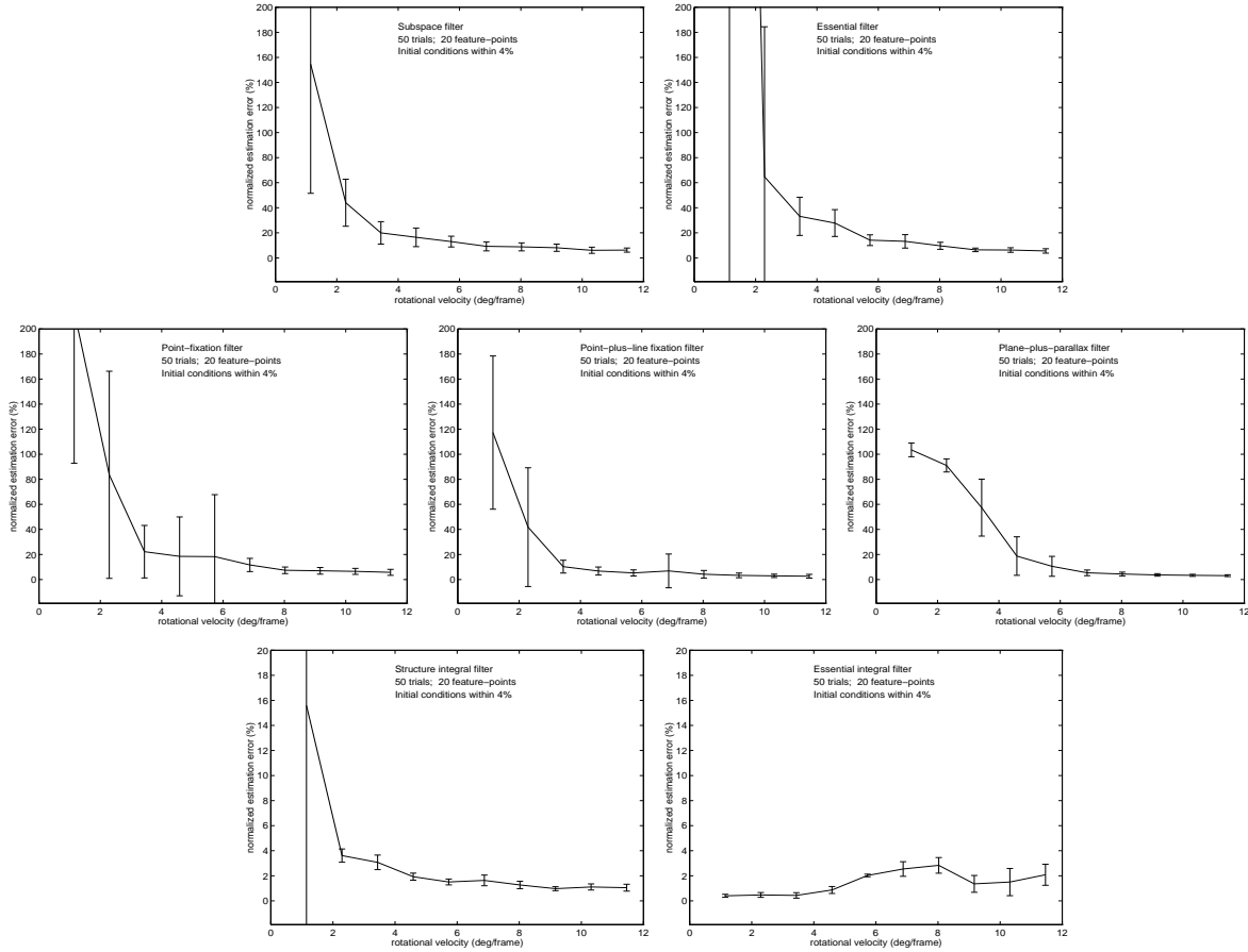
Figure 9: Dependence upon the sampling rate. The subspace filter (top-left), which is based upon a differential model, converges for smaller velocities. In principle its performance should degrade as such velocity increases, since image velocities are approximated by first differences. However, the exponential coordinatization helps maintaining good performance even in the presence of large image-motions. The performance of the integral essential filter is somewhat odd. Since the filter is based upon a second-order model, and therefore it can count on an increasingly large baseline, it can handle small motions quite well. However, when the instantaneous baseline increases, the bias in the estimate of scale increases, which causes a degradation of the performance.
