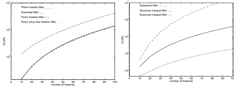
Figure 11: Complexity: number of floating point operations as a function of the number of visible features. This count includes the overhead of our Matlab implementation. The subspace filter has been implemented using a tensor package that does not exploit the sparse structure of the matrices involved in the computation.
