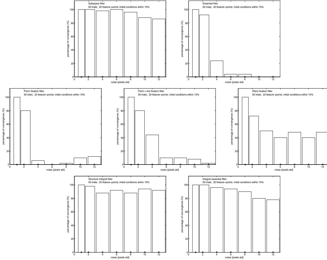
Figure 4: Robustness experiment. 50 trials with the initial conditions distributed at random within 10% of the true value, and the noise level increased from 1 to 12 pixels std. The histograms represents the percentage of the experiments in which the filters reached convergence. Integral filters (bottom row) exhibit better robustness properties than reduced filters, with the exception of the subspace filter (top-left).
