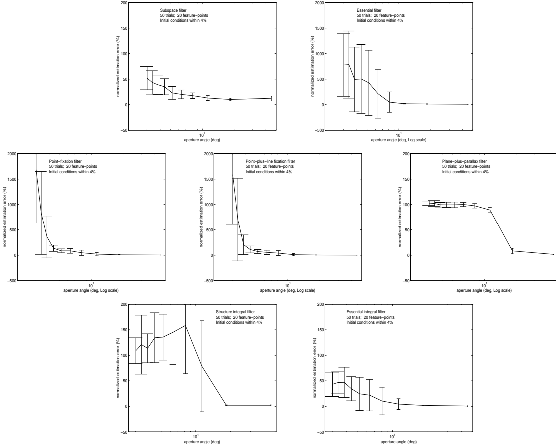
Figure 7: Dependence upon the aperture angle. Norm of the estimation error as a function of the aperture angle that ranges from 2^\circ to 40^\circ .
