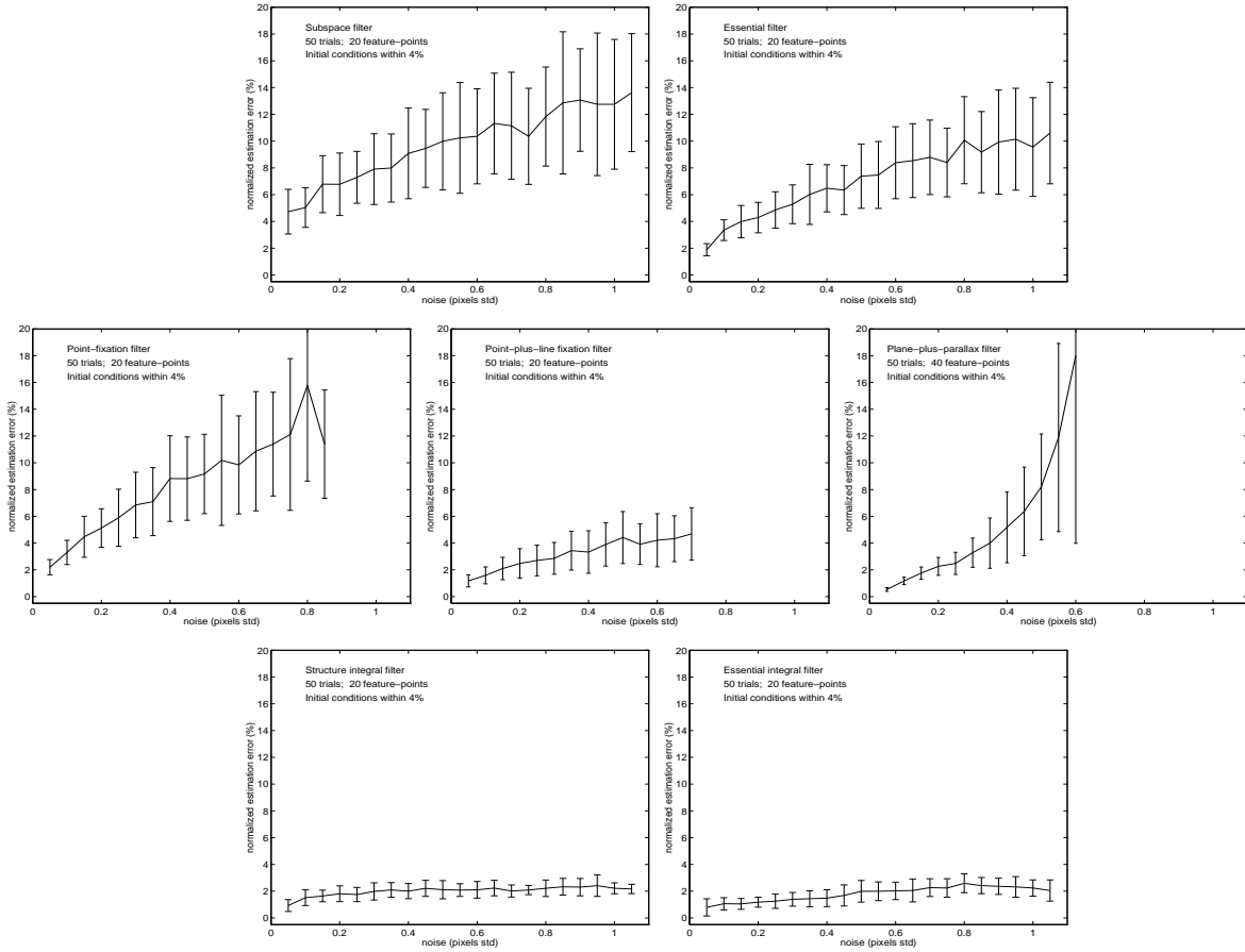
Figure 2: Accuracy experiment. 50 trials, with 20 feature-points (except for the plane-fixation filter, see also figure 6), starting at initial conditions distributed at random within 4% of the true parameters while the noise level increases from 0.1 to 1.1 pixels std, according to the standard performance of feature tracking algorithms. The scaled norm of the estimation error is plotted against the noise level. The filters enforcing a fixation constraint (middle row), cease converging consistently for less than one pixel noise. Note that integral filters (bottom row) have an advantage in performance, since they can count on an increasingly large baseline. For the integral structure filter we display only the error in the estimates of motion parameters.
