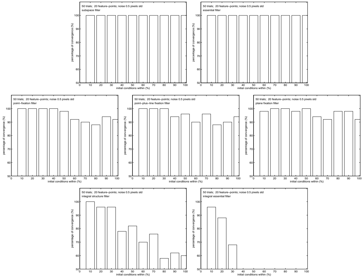
Figure 5: Convergence experiment. 50 trials with 0.5 pixel std error, while the initial conditions are chosen at random with Gaussian distribution with \sigma ranging from 10% to 100% of the true parameters. Integral filters (bottom row) exhibit decreased robustness relative to reduced filters. For the structure integral filter (bottom-left) this is mainly due to the observability properties of the model having structure in the state, while for the integral essential filter (bottom-right) this behavior is due to the mechanism of propagation of scale over time.
